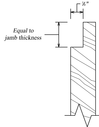
Jamb Leg Notch Detail (side view)
