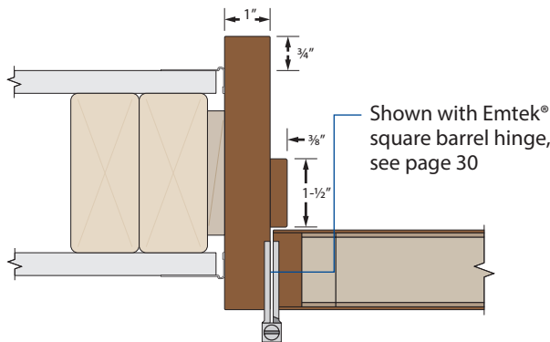
Jamb detail with Z-reveal trim and barrel hinge
