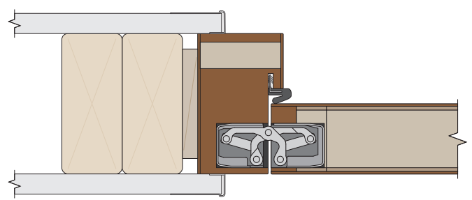
Jamb detail with L-bead trim and concealed hinge
