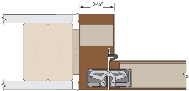
Jamb detail with L-bead trim and concealed hinge This option is available for 20-minute house-to-garage, natural wood door applications. Minimum wall depth and self-closer may be required.
