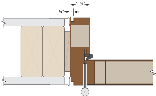
Jamb detail with L-bead trim and barrel hinge This option is available for 20-minute house-to-garage applications; minimum wall depth applies.
