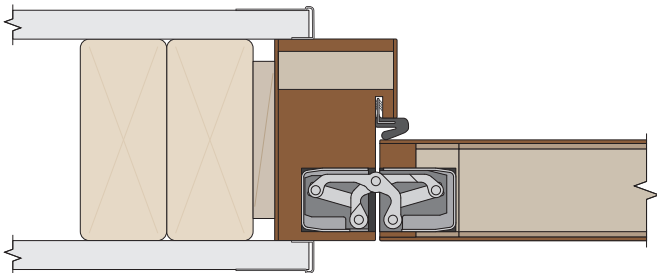
Jamb detail with L-bead trim and concealed hinge This option is available for 20-minute house-to-garage, natural wood door applications. Minimum wall depth and self-closer may be required.
