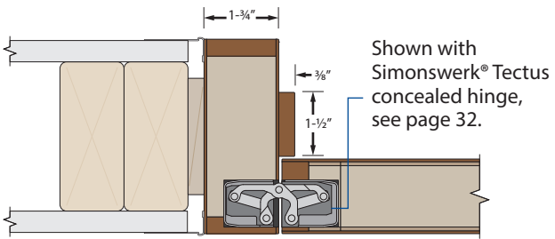
Jamb detail with L-bead trim and concealed hinge Also available in single rabbet configuration, see page 24
