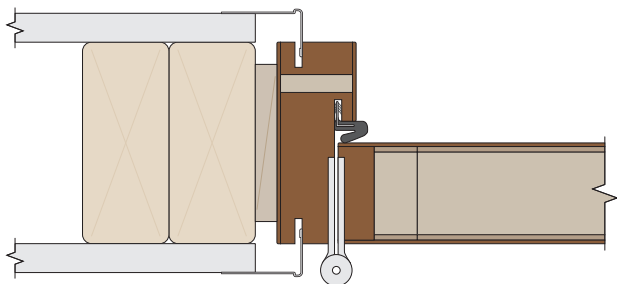
Jamb detail with L-bead trim and barrel hinge This option is available for 20-minute house-to-garage applications
