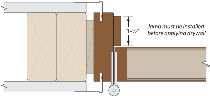
Jamb detail of drywall return jamb with barrel hinge Shown with drywall kerf
