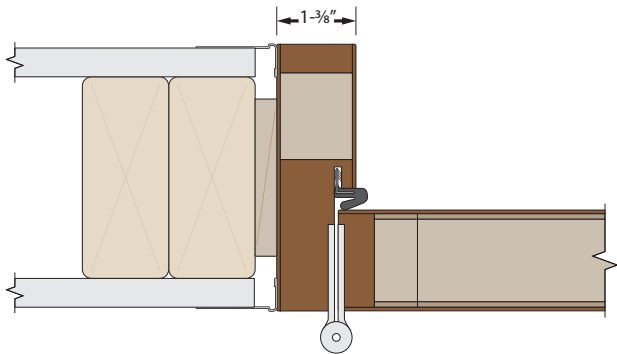
Jamb detail with L-bead trim and barrel hinge This option is available for 20-minute house-to-garage applications
