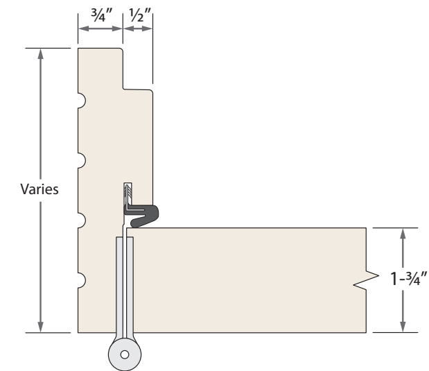
20-Minute, Double Rabbet Jamb with Square Edge Bevel edge with radius available
