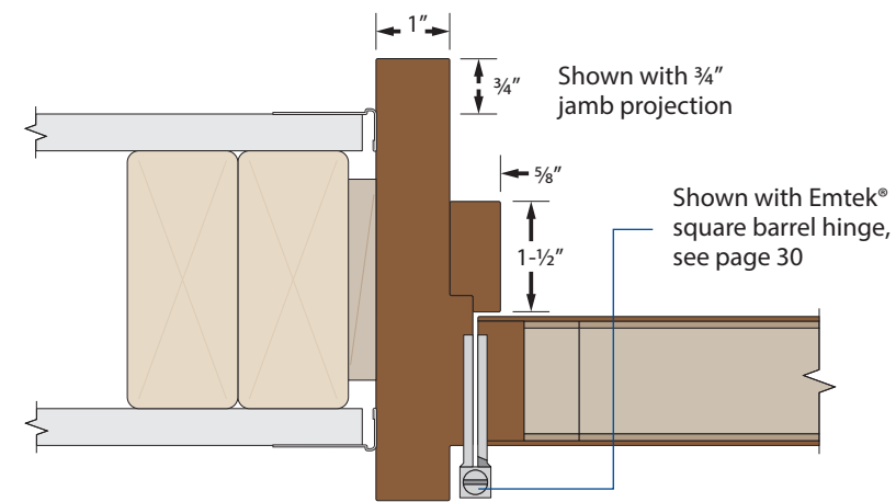
Jamb detail with L-bead trim and barrel hinge
