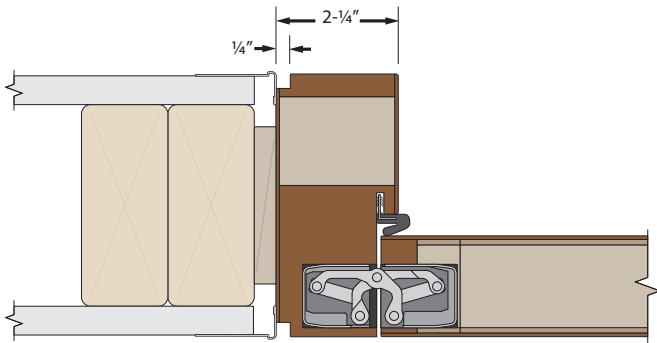
Jamb detail with L-bead trim and concealed hinge This option is available for 20-minute house-to-garage, natural wood door applications. Minimum wall depth and self-closer may be required.
