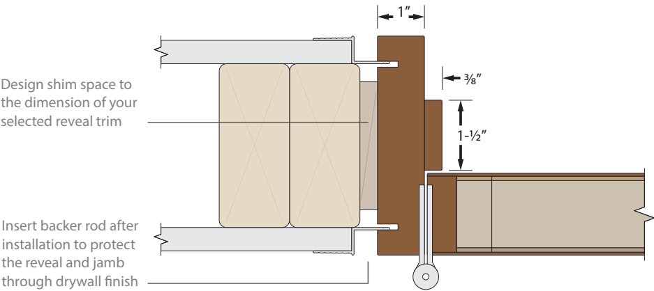
Jamb detail with Z-reveal trim and barrel hinge Also available in single rabbet configuration, see page 24. Backside kerf requires minimum 1" thickness. A similar look can be obtained, without backside kerf, with a flush-to-wall jamb with reveal, see page 21
