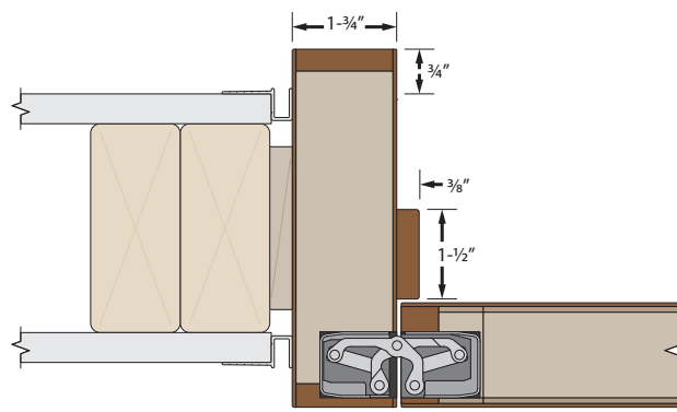
Jamb detail with F-reveal trim and concealed hinge
