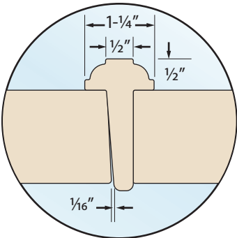
Traditional T-Astragal
