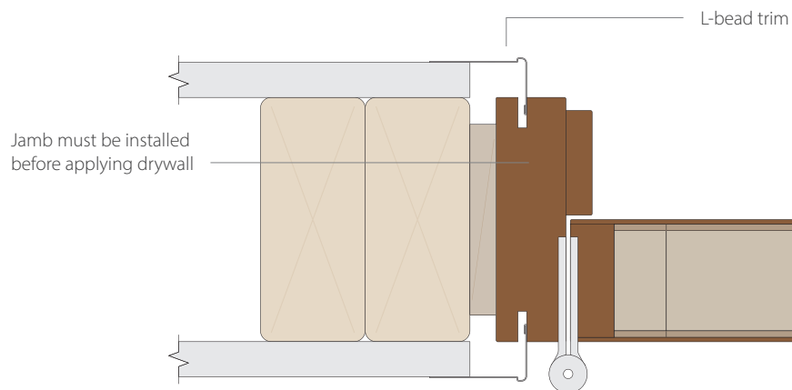
Jamb detail of drywall return jamb with barrel hinge
