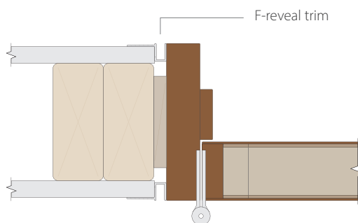
Jamb detail with F-reveal trim and barrel hinge
