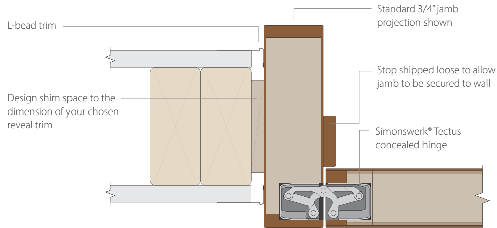
Jamb detail with L-reveal trim and concealed hinge
