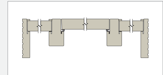
Single Rabbet Frame with 4-9/16" Uniframe Mull Posts
