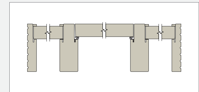
Single Rabbet Frame with 6-9/16" Uniframe Mull Posts
